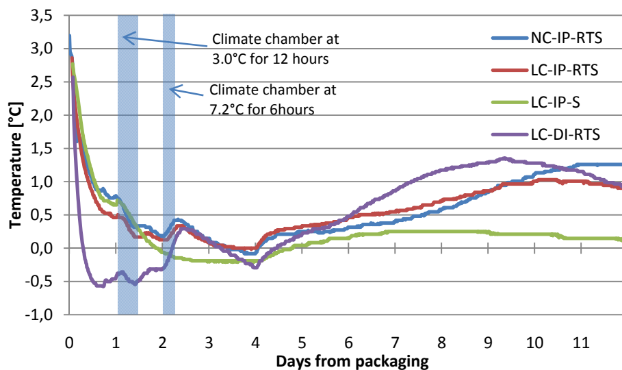
Figure 11: Average temperature history of all the groups during transportation and storage at Mafis facilities.
